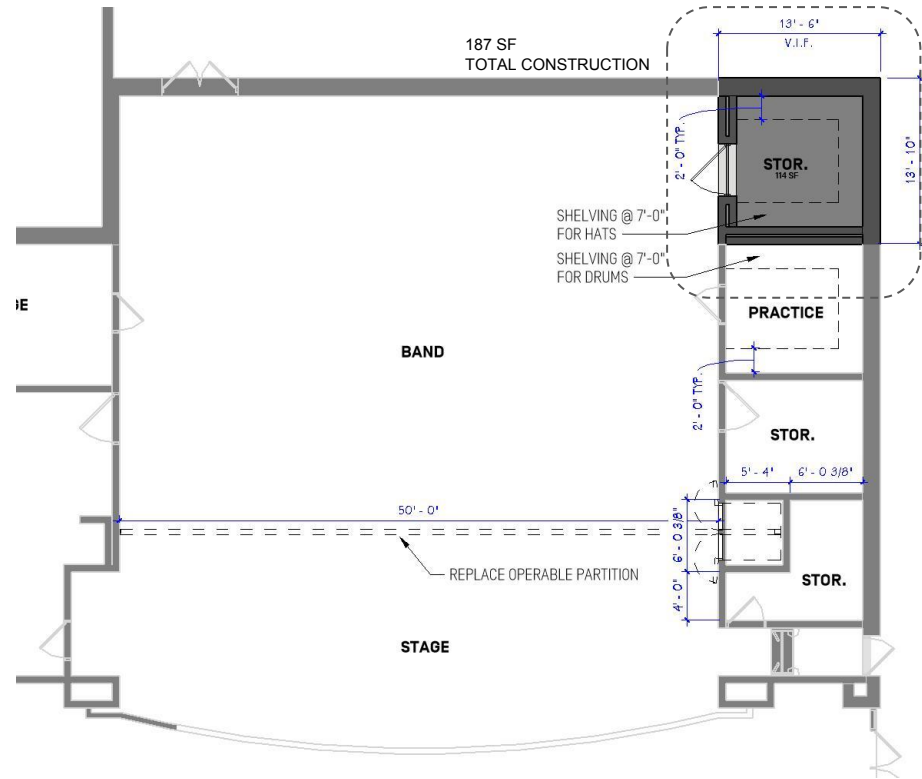
ENLARGED JR / SR HIGH SCHOOL FLOOR PLAN
