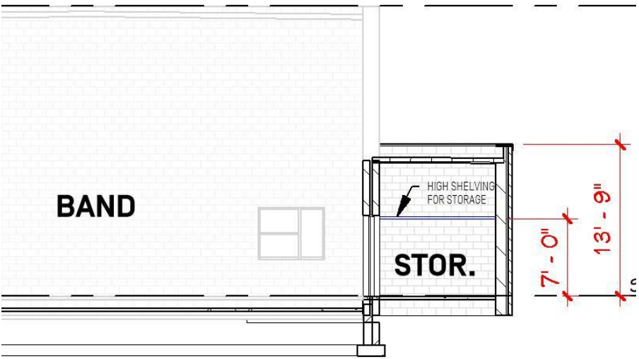
ENLARGED MUSIC STORAGE ROOM SECTION
